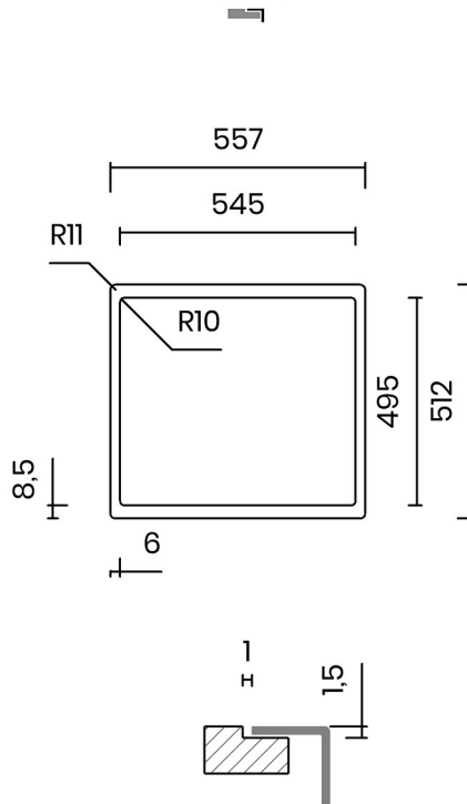
FILOTOP Flushmount
