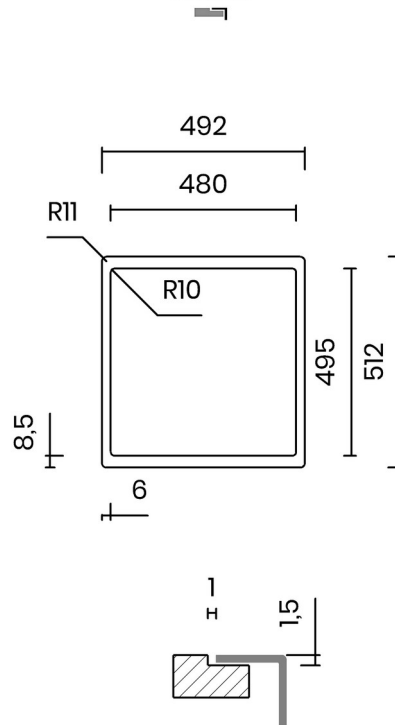
FILOTOP Flushmount
