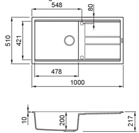
Technical Drawing
